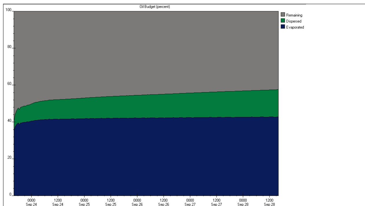
Figure 6-5 Predicted Fate and Weathering for a continuous release of 1.6 m 3 /d
